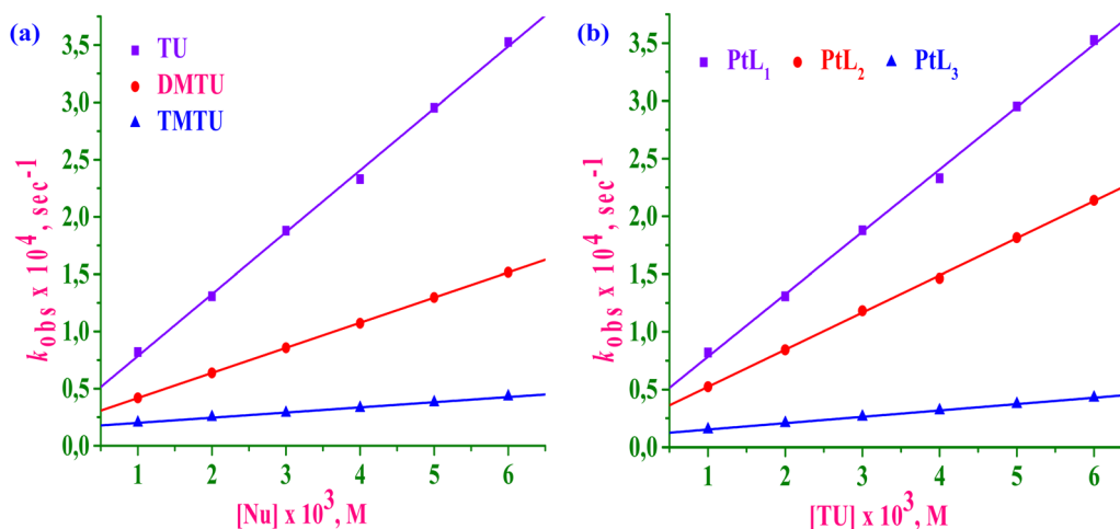
Fig. 2 Linear plots of k_{\text{obs}} versus [Nu] for the reaction of PtL 1 with Nus (a) and for the reactions with three Pt(II) C \wedge N \wedge C pincer complexes ( PtL 1 , PtL 2 and PtL 3 ) with Tu (b): [ PtL 1 / PtL 2 / PtL 3 ] = 50 \mu M, pH = 7.2 (5 mM Tris-HCl/50 mM NaCl) and T = 35 ^{\circ} C.
